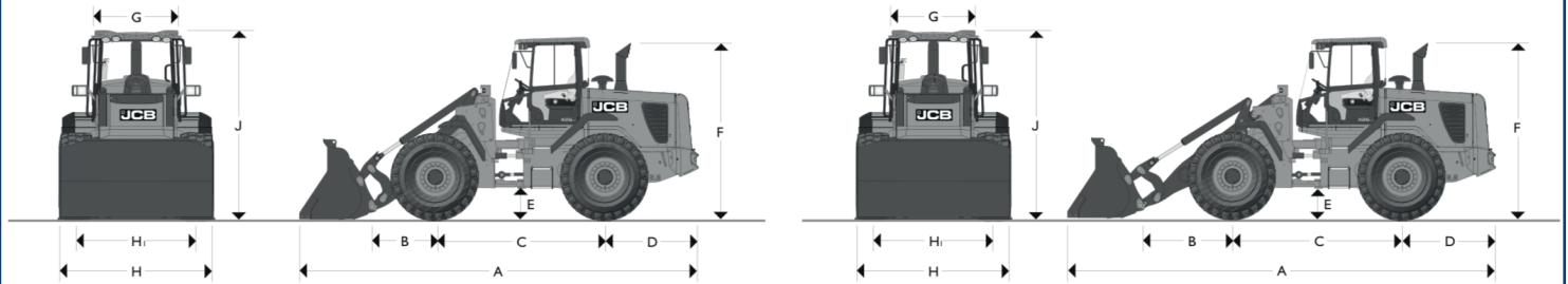
426/426e HT – STATIC DIMENSIONS – Standard height arm
