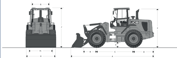
426/426e ZX – STATIC DIMENSIONS
